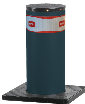
RANCH C Ø275/600-800 RANCH C Ø275/600-800 INOX
